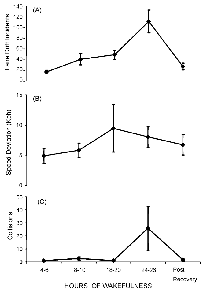
Fig. 2. Mean driving performance data, demonstrating the effects of extended wakefulness on (Panel A) lane drifting; (Panel B) speed deviation and (Panel C) collisions.
