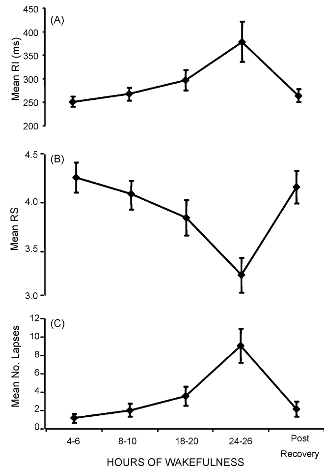
Fig. 3. Mean PVT data, demonstrating the effects of extended wakefulness on (Panel A) reaction time (ms); (Panel B) response speed (1/RT), and (Panel C) number of lapses (RT > 500 ms).
